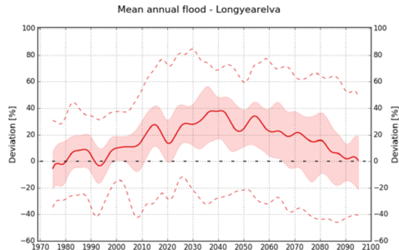
Figure 10.2.3. Mean annual flood for the river Longyearelva, simulated using the HBV-model forced with down-scaled and bias-adjusted Arctic CORDEX data for the high emission scenario RCP8.5. The solid red line shows the ensemble median of eight models; the pink band outlines the 25th and 75th percentiles, whereas the dotted lines indicate the minimum and maximum. Flood values are given as deviation (%) from the reference period 1971–2000. The low-pass filtered series are smoothed by Gaussian weighting coefficients, and show variability on a decadal time scale.
