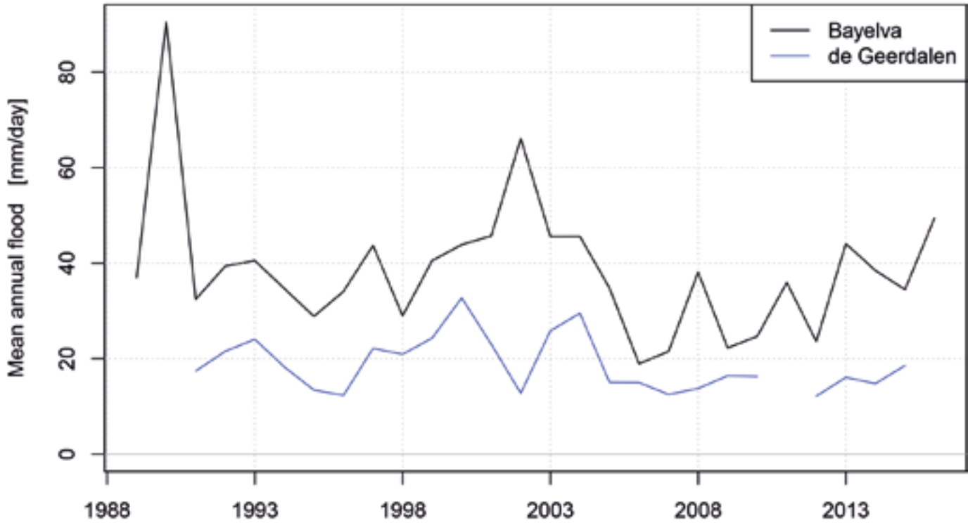
Figure 5.1.10 Historical annual maximum streamflow at the two runoff stations in Svalbard.
