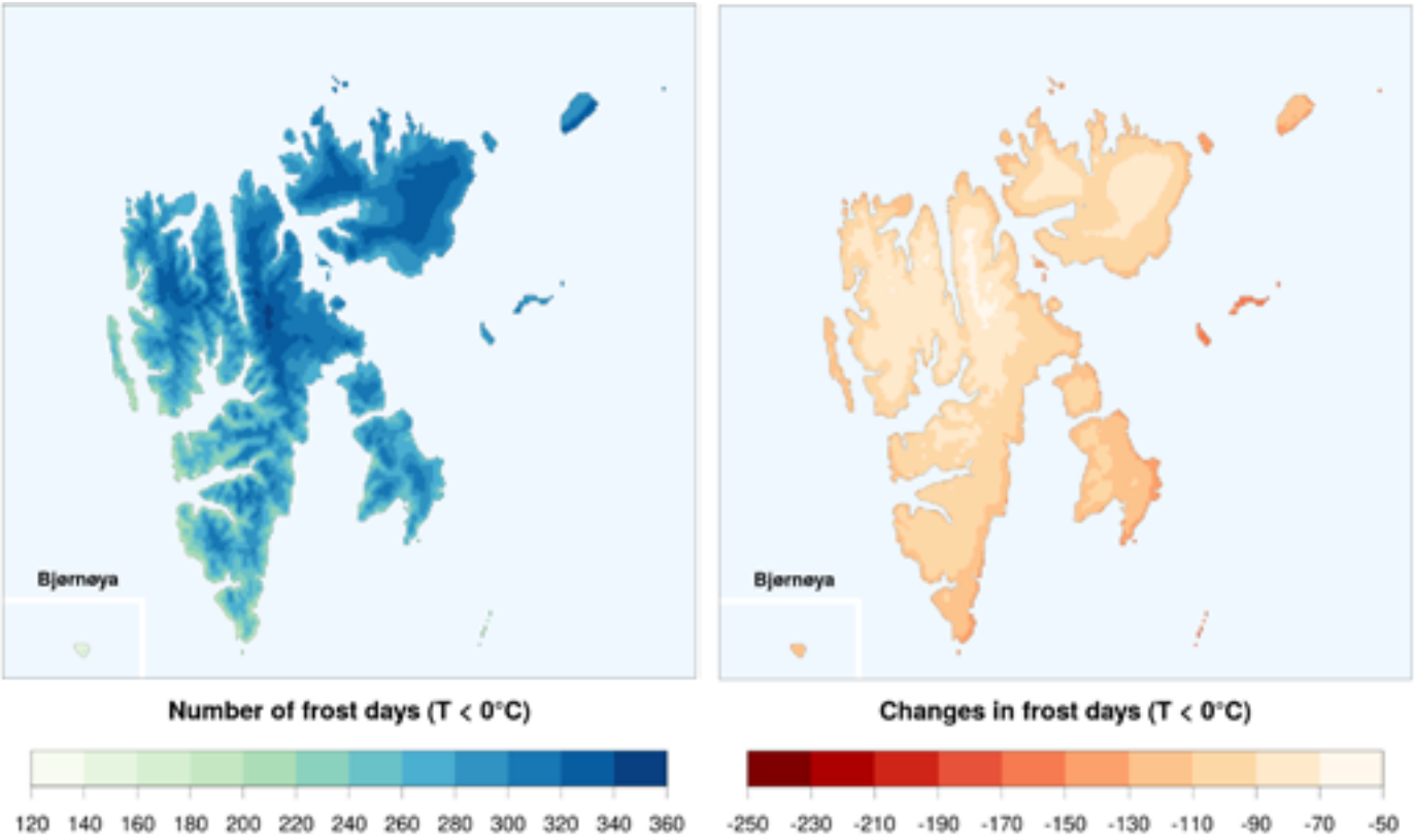
Figure 4.2.2: Average number of frost days per year in the control period 1971-2000 (left), and projected change from 1971-2000 to 2071-2100 (right) according to CCLM under the RCP8.5 emission scenario.
