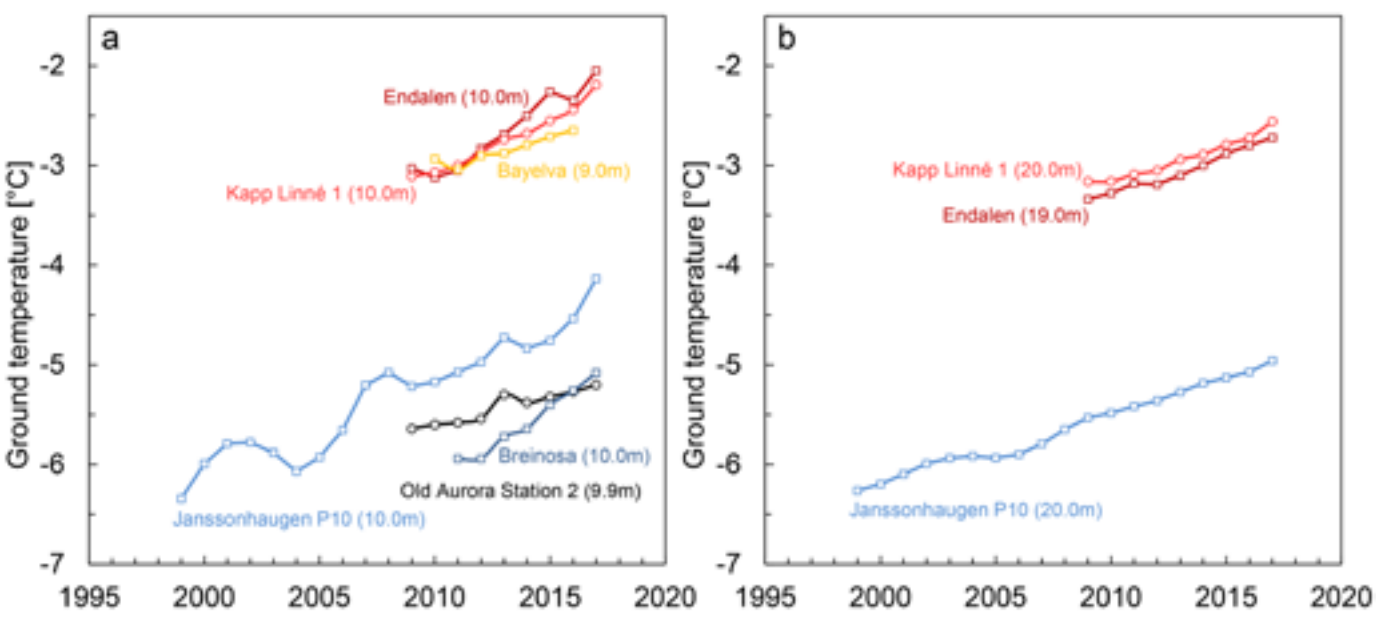
Figure 7.1.2 Annual mean ground temperatures (MGT) during hydrological years at selected permafrost monitoring sites on Svalbard. a) 10 m below the surface and b) at 20 m depth, near or at the depth of zero annual amplitude (ZAA), only available from Janssonhaugen, Kapp Linné and Endalen. Data series are updated from Isaksen et al. 2007a, Christiansen et al. 2010 and Boike et al. 2018.
