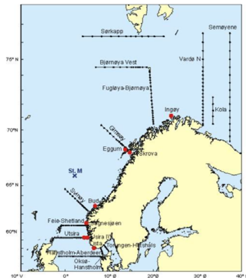
Figure 3.5.1 Map of fixed stations and sections with regular observations of hydrographic variables. Red dots show coastal stations with regular observations, and the blue cross shows the location of Ocean Weather Ship Station Mike (OWS M) at ( 66^{\circ} N, 02^{\circ} E), and the new buoy to observe currents, hydrography and biogeochemical properties.
