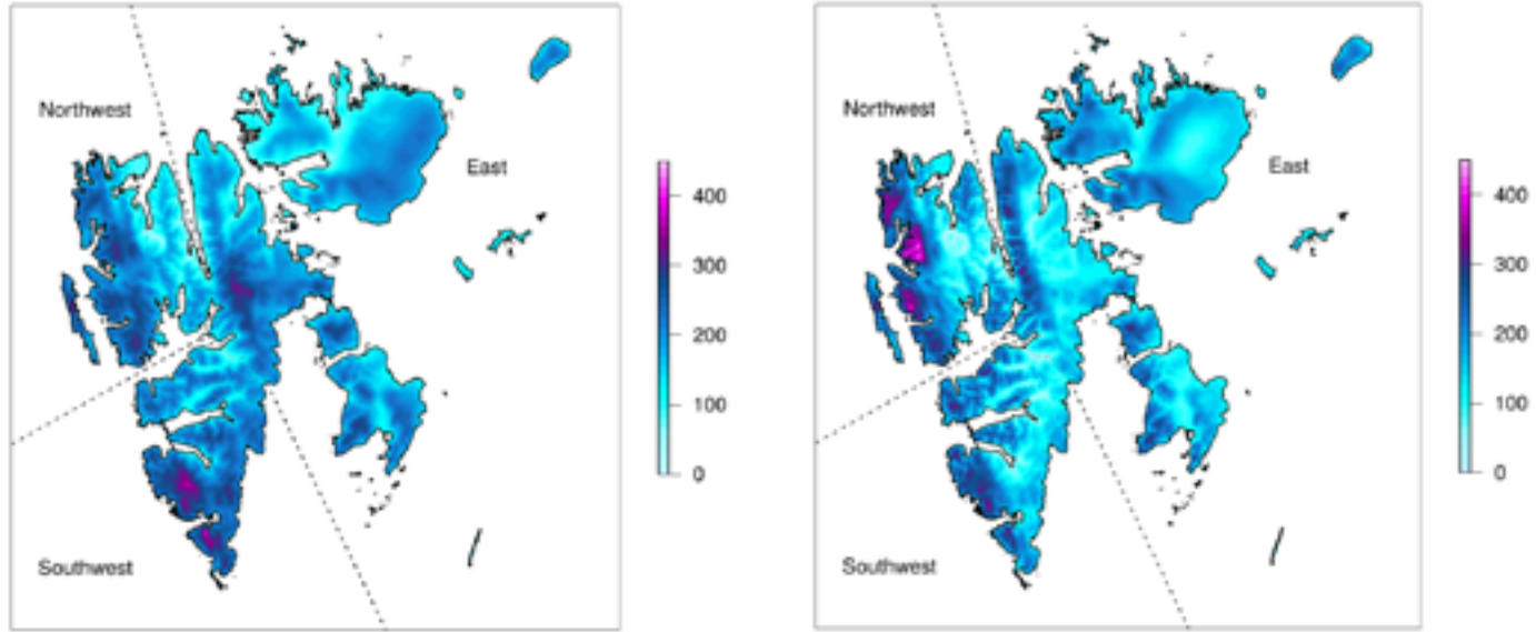
Figure 4.3.2. Downscaled precipitation [mm] for the reference period 1971-2000. Left: Winter (Dec-Jan-Feb), right: Summer (Jun-Jul-Aug)
