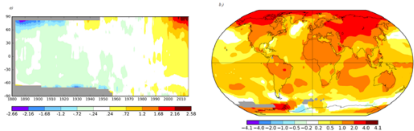
Figure 2.3.1: 5-years zonal mean temperature anomalies (°C) compared to the 1961-1990 normal (a) and temperature trends (°C) from 1950-2017 (b). Data from NASA Goddard Institute for Space Studies (NASA GISS).
