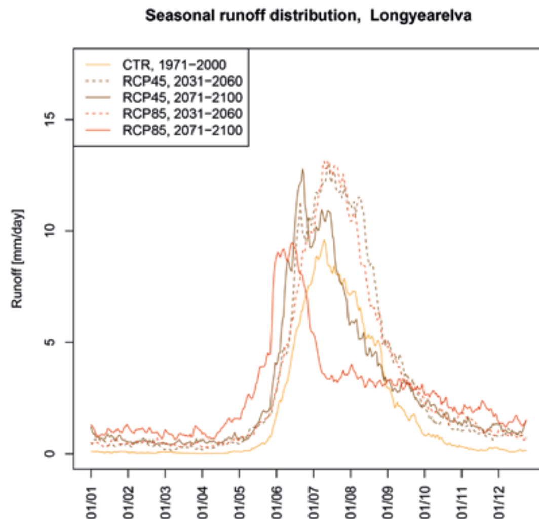
Figure 10.2.2. Modelled seasonal distribution of the Longyearelva runoff for the periods 1971–2000, 2031–2060 and 2071–2100.
