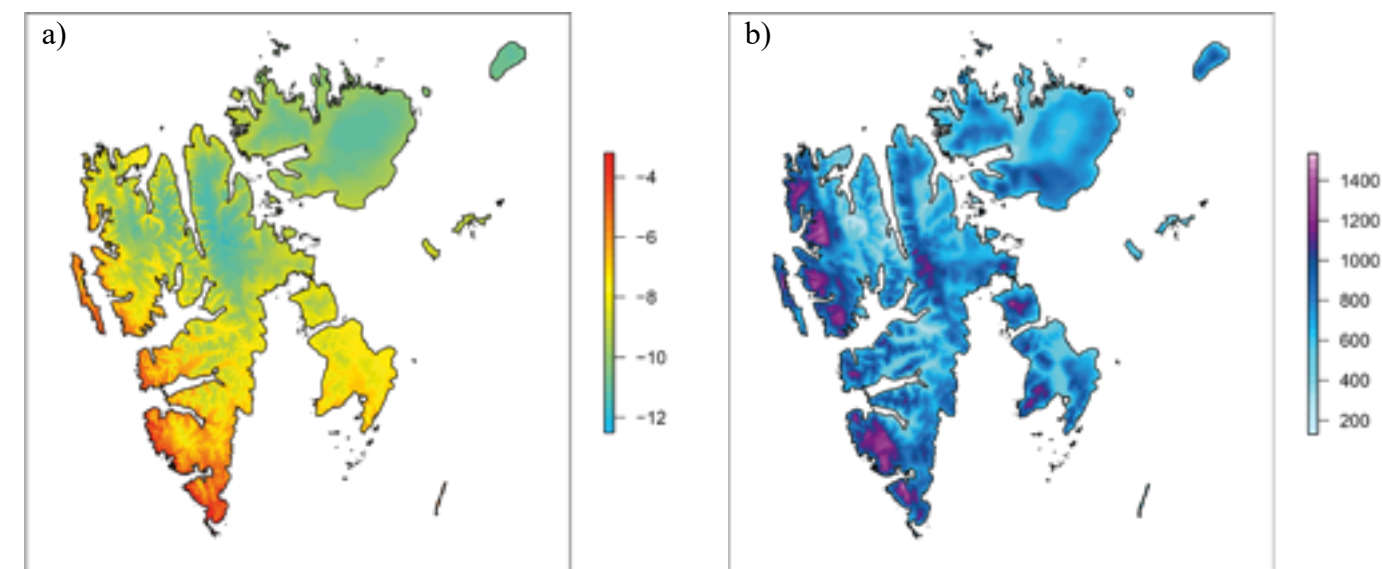
Figure 2.1.2. Downscaled annual temperature (°C; a) and precipitation (mm; b) from the Sval-Imp dataset (Østby et al., 2017) averaged over the period 1971-2000. Seasonal maps for summer and winter are found in Chapter 4.
