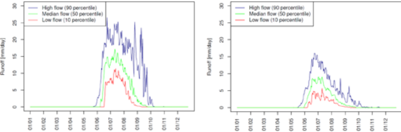
Figure 5.1.1 Seasonal cycle at Bayelva (1989–2017) and De Geerdalen (1991–2015).
